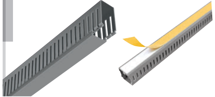
BL-1766 BL-1768 (Adhesive) (Nonviscid Adhesive) 100x60 Perforated Cable Duct ترنكات الكابلات المثقبة 100x60
